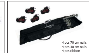
stake kit (inclusive with each Dome)
