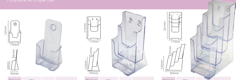
Leaflet 1/3 A4 Polystyrene Dispenser
