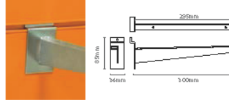
300mm Shelf Bracket (left and right)
